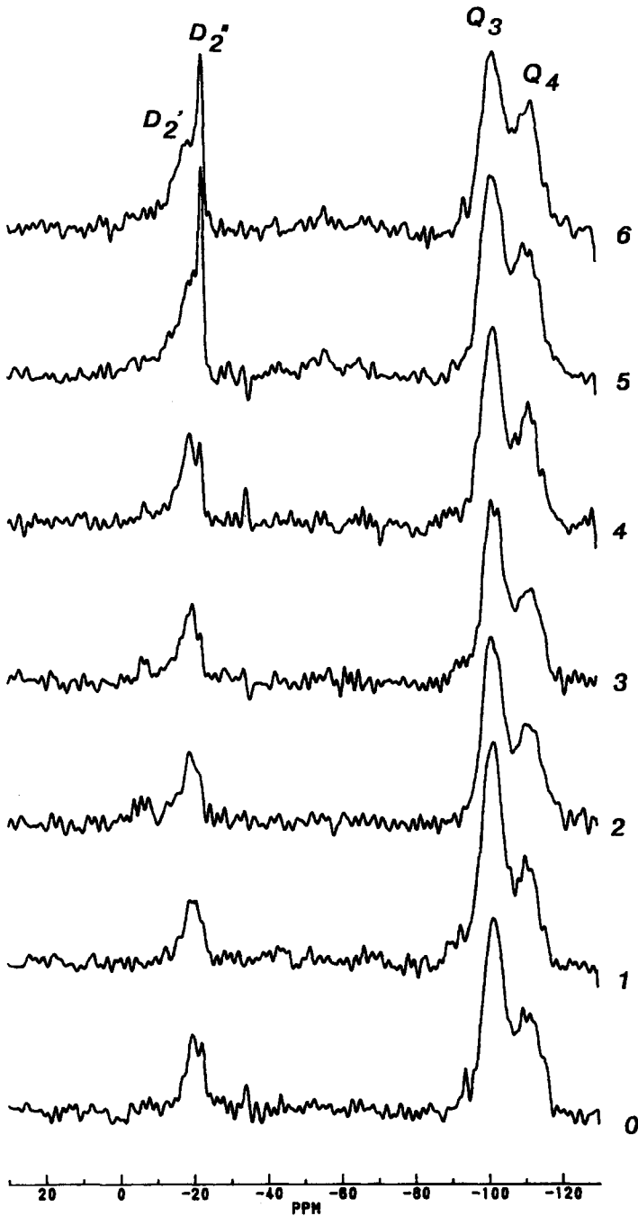
Fig. 8. ^{29}\text{Si} CP-MAS NMR spectra of the PMSC 18 phases before (expt. 0) and after the ageing experiments. Conditions as in Fig. 6.
